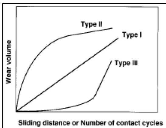
Fig 1: Three Representative Types of Wear Curves in Repeated Contacts
