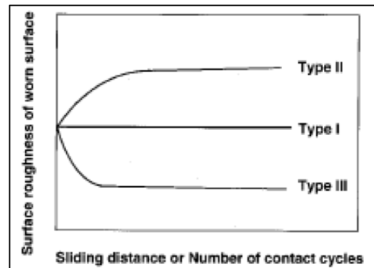
Fig 2: Three Representative Types of Surface Roughness Changes in Repeated Contacts
